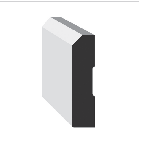
T-C4326 11/16" X 2-3/4" 7', 16'
